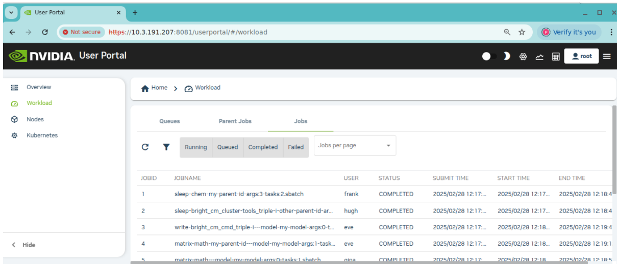
Figure 12.2: User Portal: Workload Page
